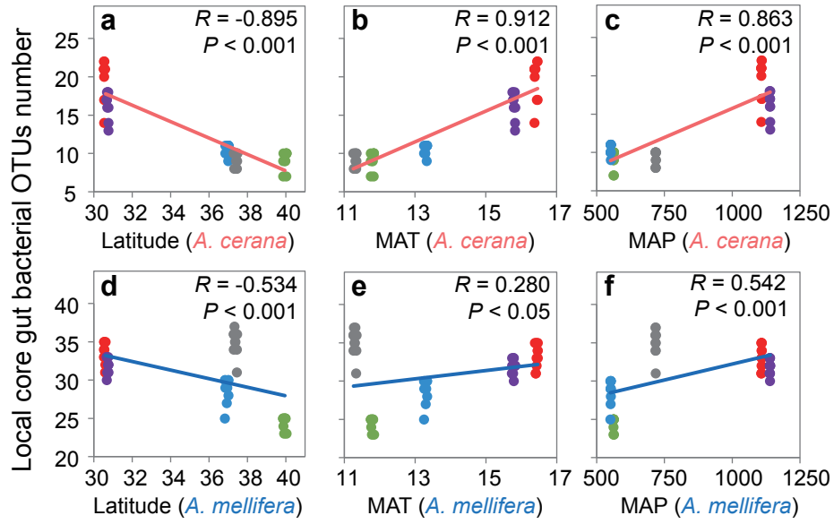
Fig. S3 Local core gut bacterial species (OTUs at 97% identity) number significantly correlates with latitude, mean annual temperature (MAT), and mean annual precipitation (MAP) for both A. cerana and A. mellifera . a-c, A. cerana . d-f, A. mellifera .
