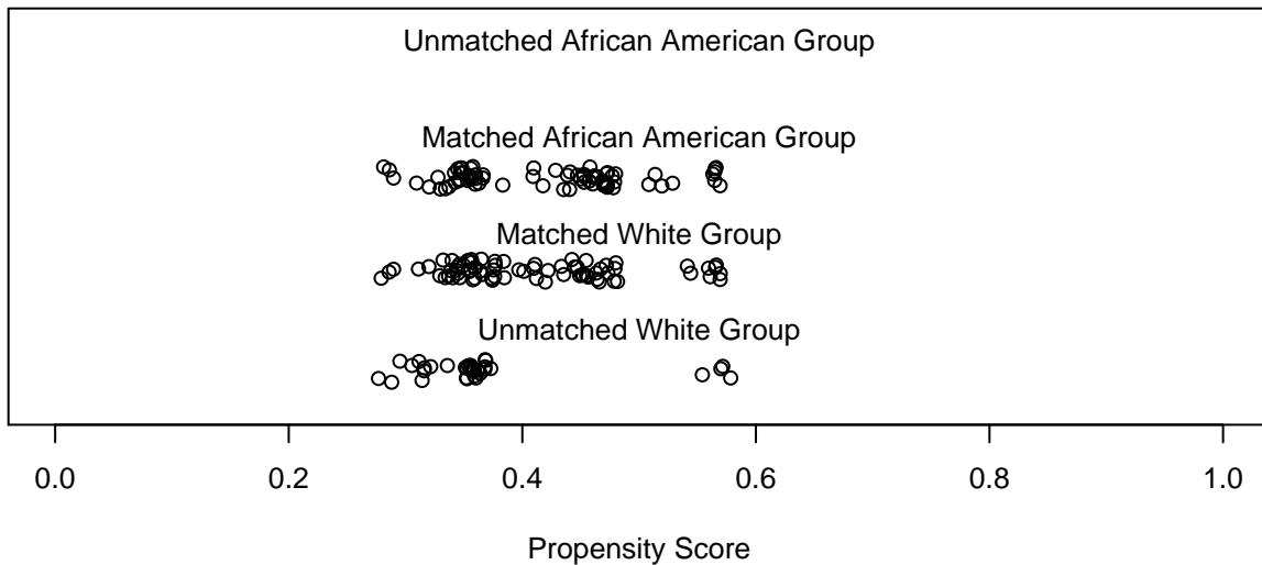
Distribution of Propensity Scores
