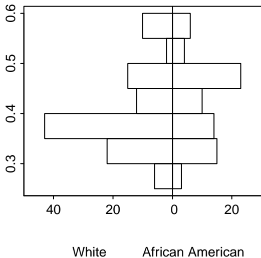
Propensity Score Before Matching
