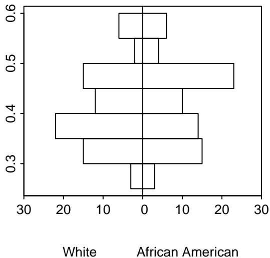
Propensity Score After Matching
