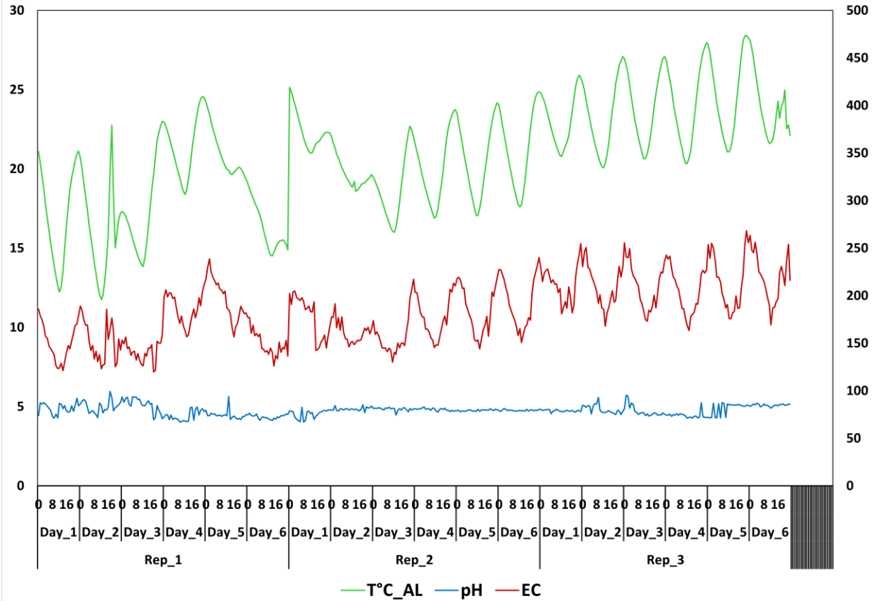
Hourly average Temperature, pH and Electrical conductivity around the roots of common bean seedlings grown under Aluminum treatment
