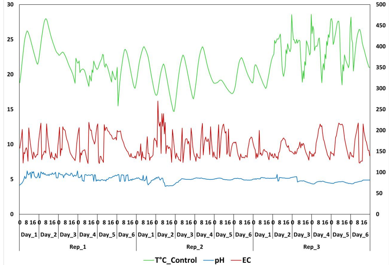
Hourly average Temperature, pH, Electrical conductivity around the roots of common bean seedlings grown under control treatment
