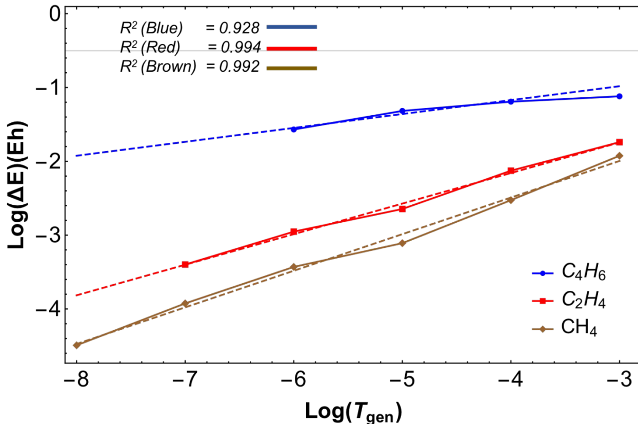
Figure 10. Fit of the errors to extrapolated FCI energies using the variational ICE energy with decreasing T_{Gen} and a fixed ratio of T_{Var}/T_{Gen} = 10^{-3} . The figure illustrates the quality of the linear fit with R^2 = 93\% , 99\% , 99\% for C_4H_6 , C_2H_4 and CH_4 respectively.
