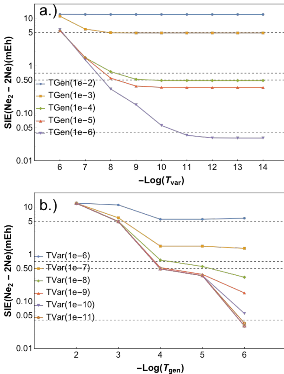
Figure 12. Size-inconsistency error (SIE) for DET-ICE variant calculated by taking the difference of Ne 2 and 2 Ne energies.
