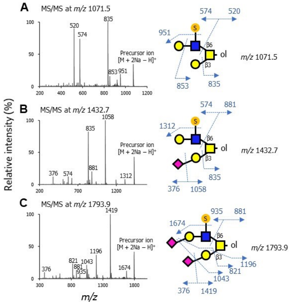
Supplementary Fig. S2 , Selected MS/MS spectra of permethylated sulfated O -glycan alditol released from ovomucin powder.
