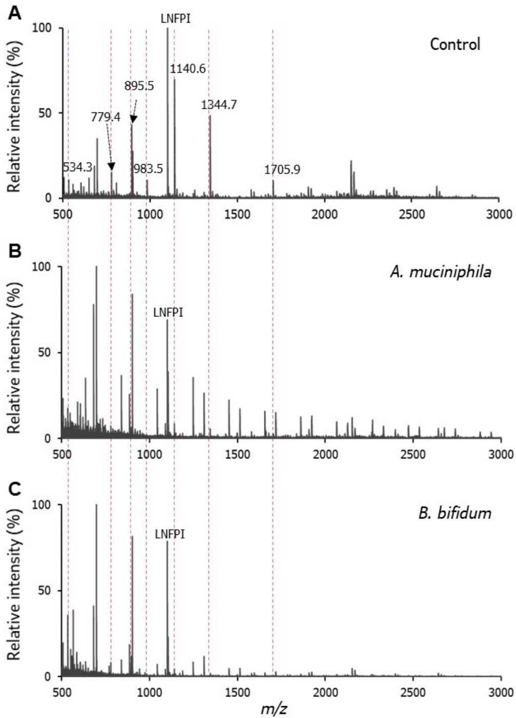
Supplementary Fig. S3 , Comparison of full mass profiles of permethylated non-sulfated O -glycan alditols released from ovomucin after the culture with mucin-degrading gut microbes.
