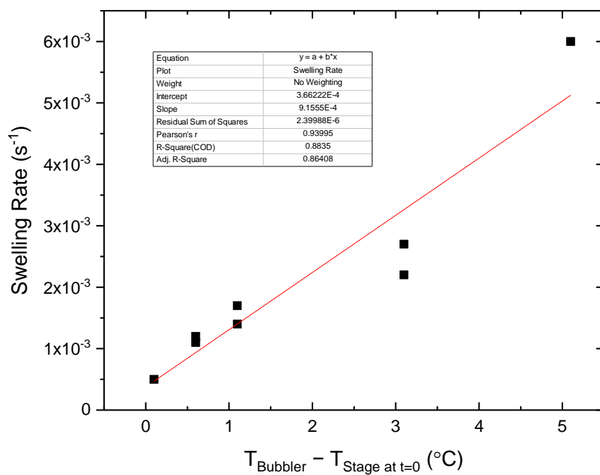
Figure S6: Plot of the calculated swelling rate vs. the difference between the initial stage temperature (varied between 15.9^\circ\text{C} to 20.9^\circ\text{C} ) and bubbler temperature ( 21^\circ\text{C} for all samples).
