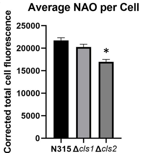
Figure S1. Quantification of NAO fluorescence in cardiolipin synthase knockout mutants ( A ) with representative images ( B ).
