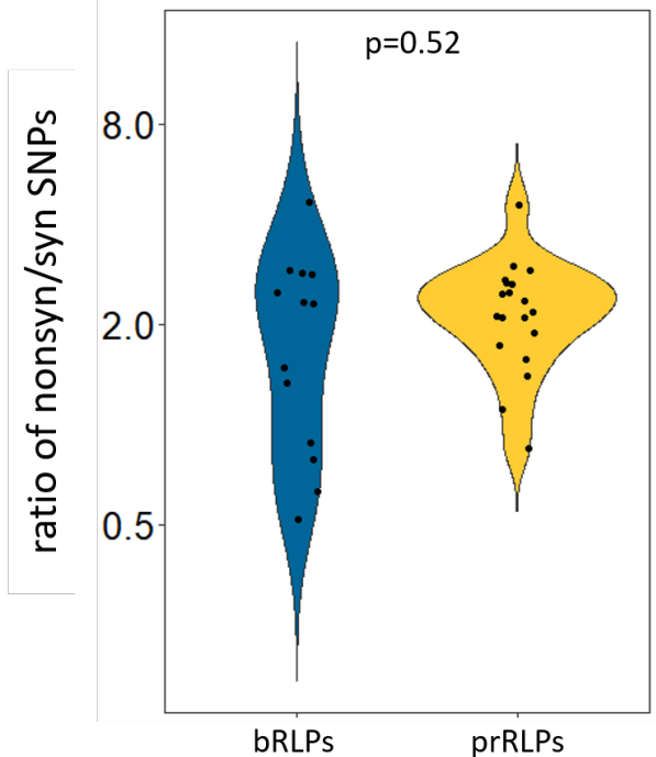
Figure S3: Ratio of non-synonymous over synonymous SNPs on a logarithmic scale (y axis) as calculated with PopGenome for the bRLPs and prRLPs (x axis).
