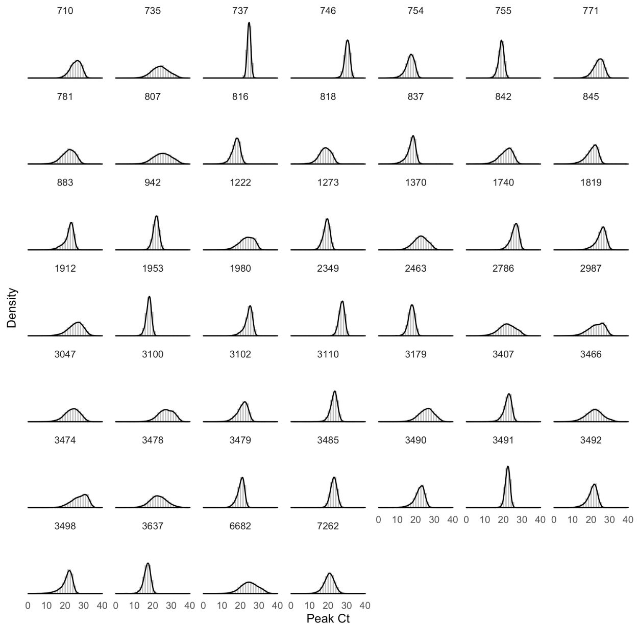
S9 Fig. Posterior peak Ct value distributions for the 46 individuals with acute infections. Underlying data are available at https://github.com/gradlab/CtTrajectories/tree/main/output/params_df_split.csv 10
