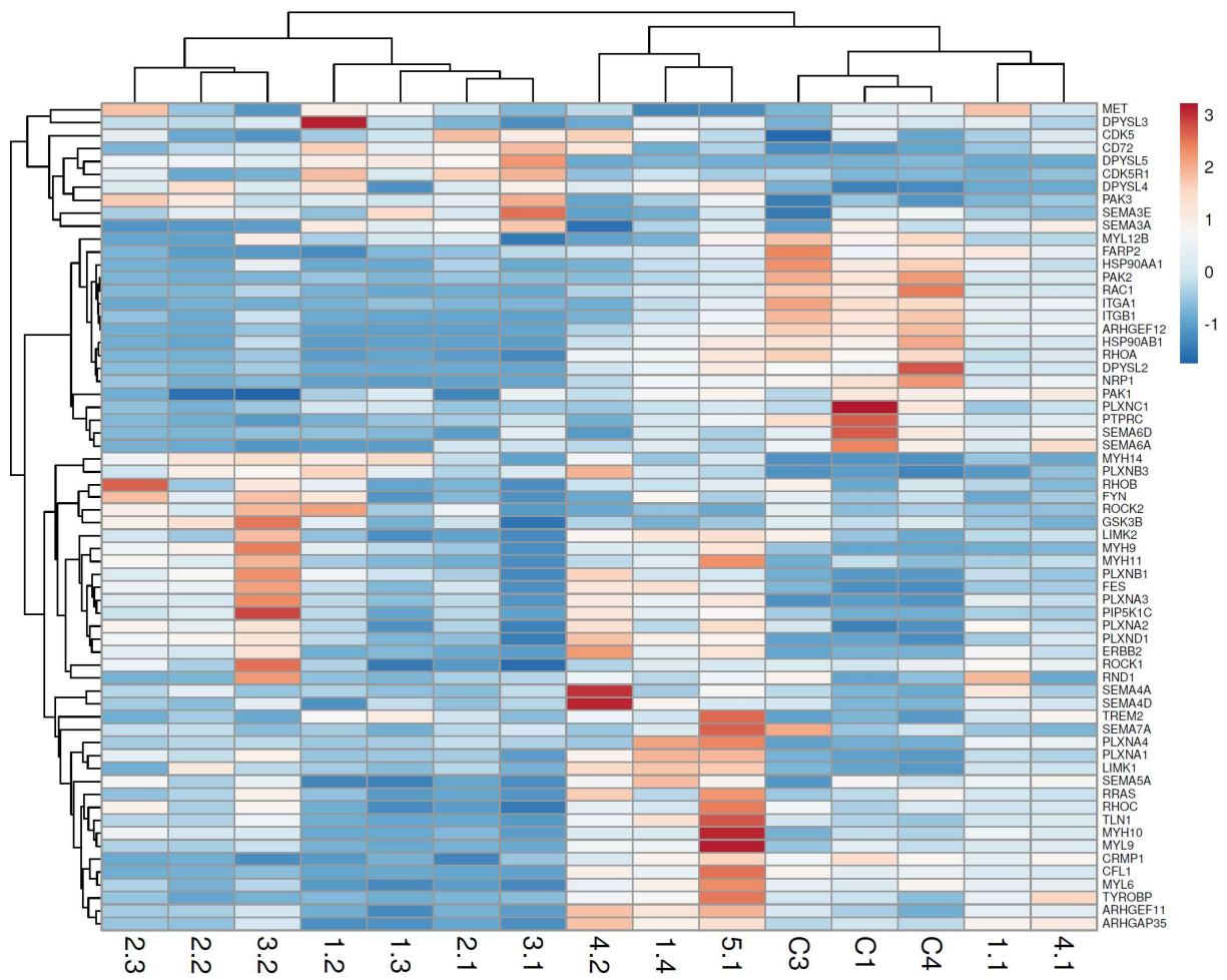
Additional file 9. Heatmap indicating hierarchical clustering of ACDMPV and non-ACDMPV control samples based on the RNA-seq expression values of genes from semaphorin interaction (R-HSA-373755).
