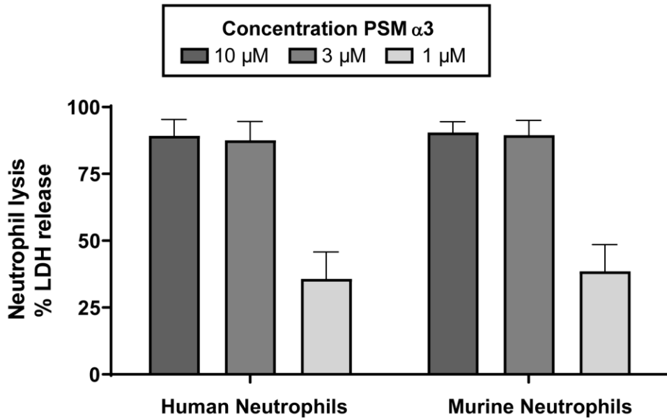
S Figure 1: No difference in PSM induced lyses between human and murine neutrophils. Dose-dependent neutrophil lysis induced by synthetic PSMα3. Neutrophils were isolated from healthy human donors or murine bone marrow. Neutrophil lysis was measured via LDH release. Data represent means ± SEM of three independent experiments.
