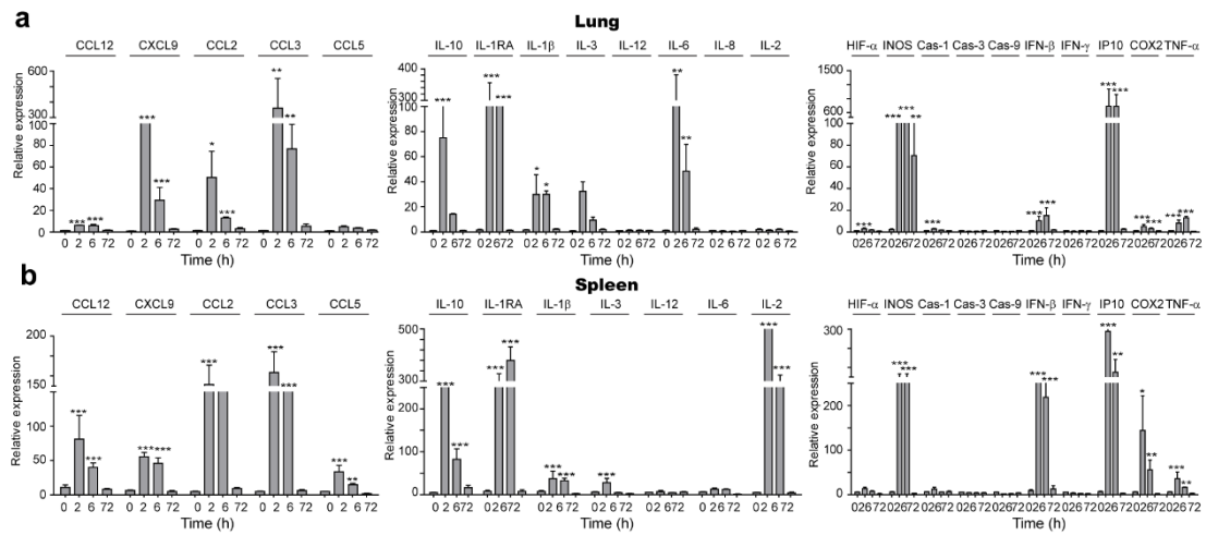
Supplementary information, Fig. S8: qRT-PCR analysis of lung and spleen tissues
