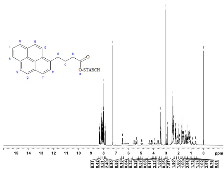
Fig.S2 1 H NMR spectrum of STARCH-PBA (FS)
