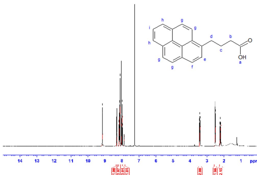
Fig.S1 1 H NMR spectrum of PBA
