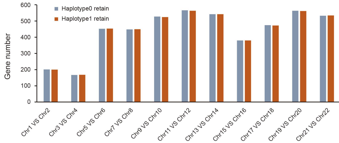
Supplementary Fig. S10 Number of single copy genes in the paired chromosomes of the two haplotypes. The allelic genes showed equivalent distribution in between the two haplotypes.
