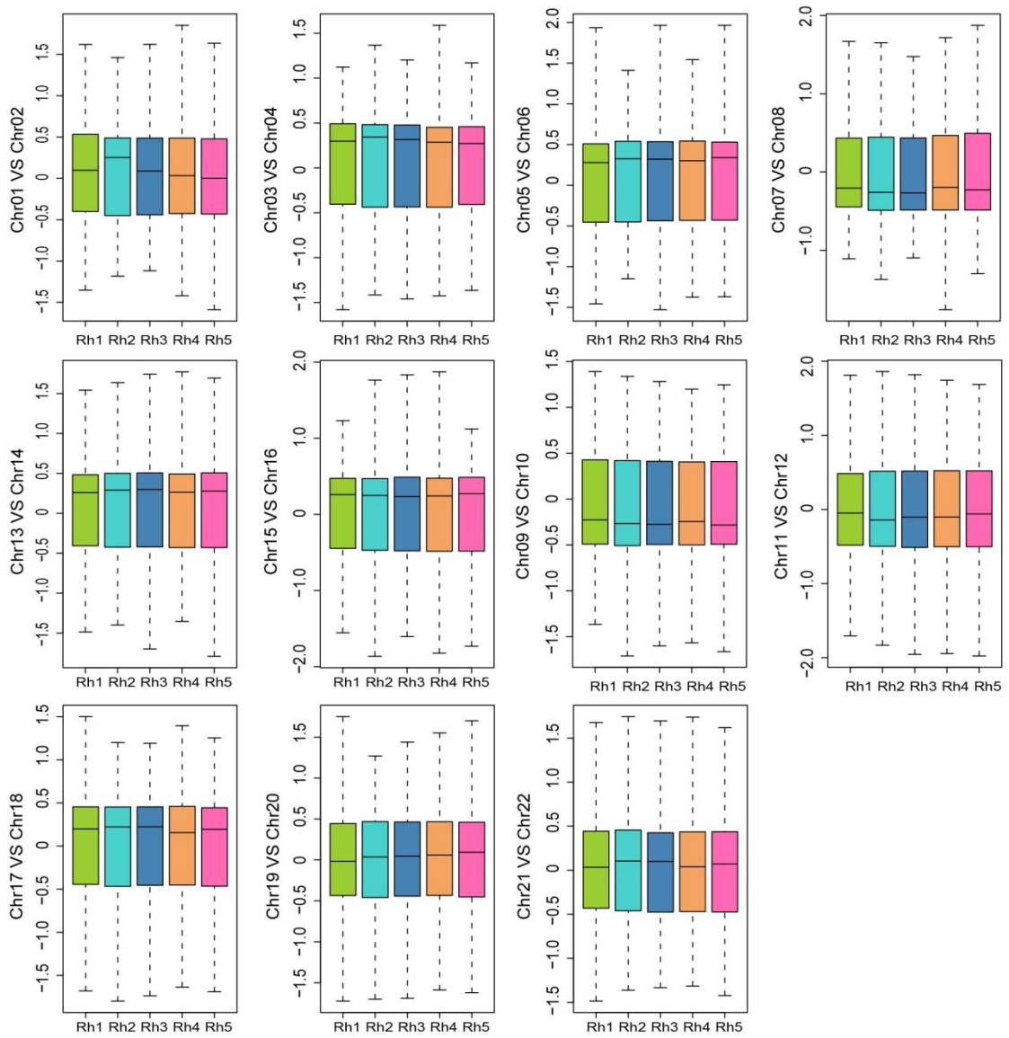
Supplementary Fig. S15 Ratio of the differentially expressed allelic genes in paired chromosomes of haplotype 0 and haplotype 1.
