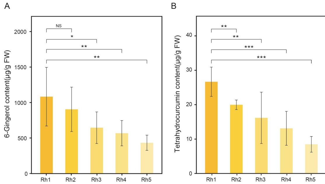
Supplementary Fig. S23 The concentration of 6-gingerol (A) and tetrahydrocurcumin (B) in ginger rhizomes by using triple quadrupole mass spectrometry. “NS” short for not significance.
