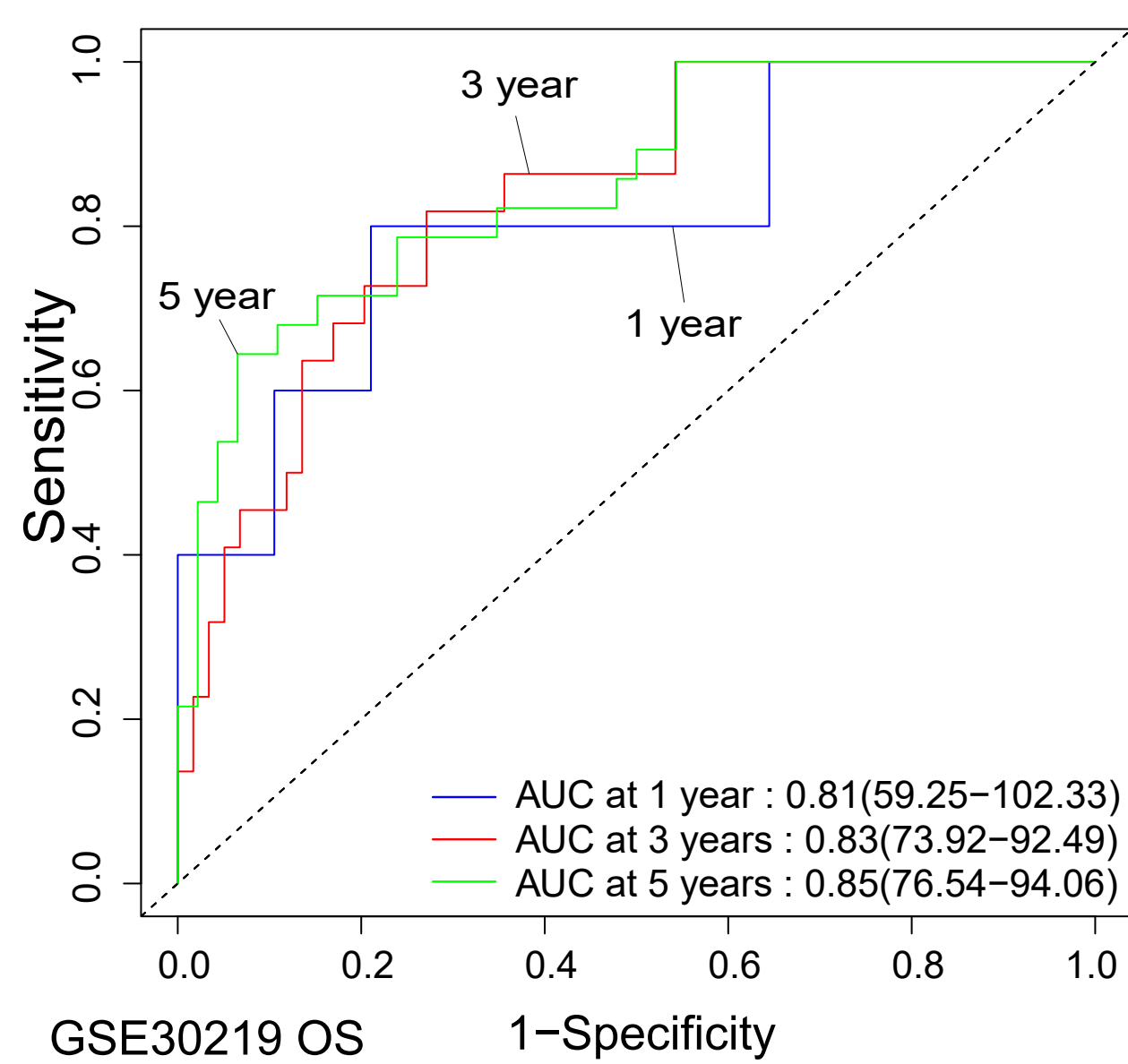
A Risk score ROC curve
