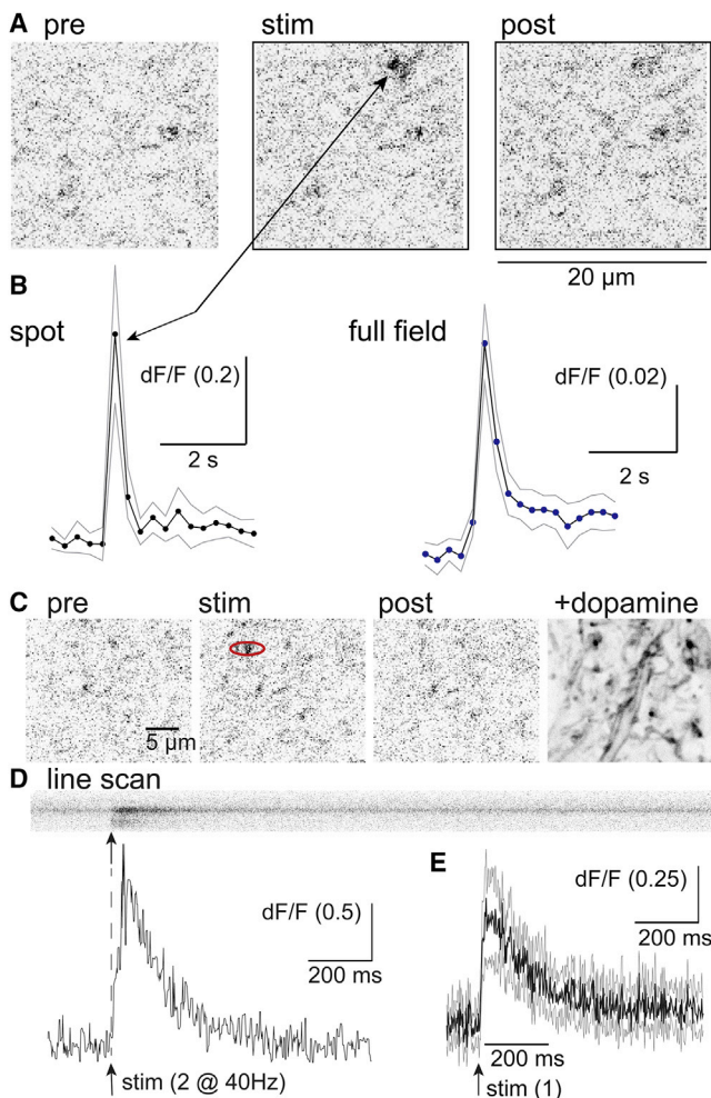
Figure 1. Location and kinetics of dopamine release measured with dLight1.3b
