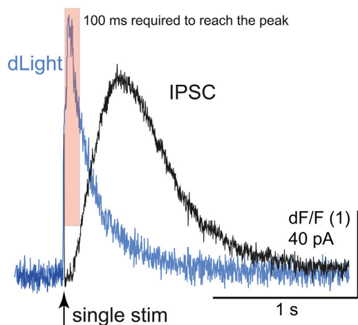
Figure 4. Illustration of the relative time course of the rise and fall of extracellular dopamine measured with dLight superimposed on the IPSC
