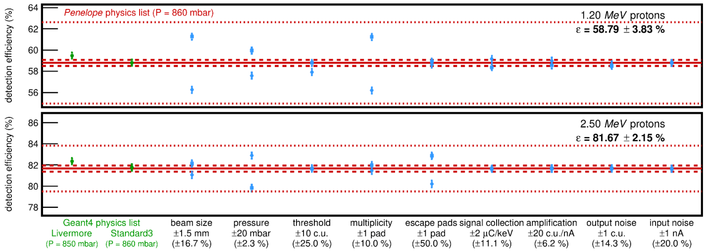
Supplementary Figure 1. Plot showing the contributions of simulation parameters to the uncertainties of the detection efficiencies
