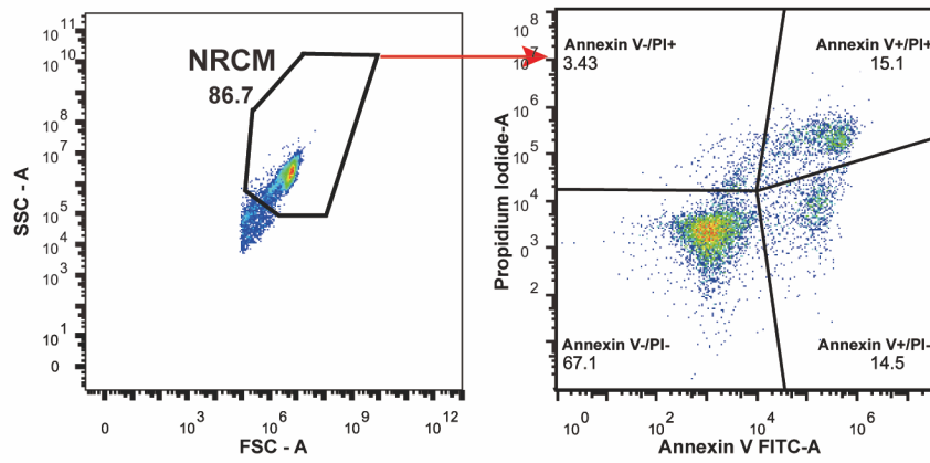
Supplementary Figure1. Sorting Strategy for the Annexin V FITC assay relate to Figure 4c. NRCM, neonatal rat cardiomyocytes; FSC-A, forward scatter-area and SSC-A, side scatter-area.
