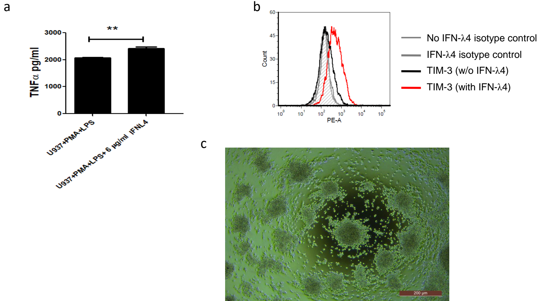
Suppl. Fig. 1: (a) TNF- \alpha secretion was measured by enzyme-linked immunosorbent assay from cell-free supernatants of U937 cells treated with PMA in the absence or presence of IFN- \lambda 4 for 48 h followed by incubation with LPS (pre-treatment strategy). (b) IFN- \lambda 4 (6 \mu g/mL)-treated THP-1 macrophage-like cells activated with LPS show increased surface expression of TIM-3. (c) Microscopic image (amplification: \times 10 ) of THP-1-derived M2 macrophage-like cells differentiated in the presence of IFN- \lambda 4 (6 \mu g/mL).
