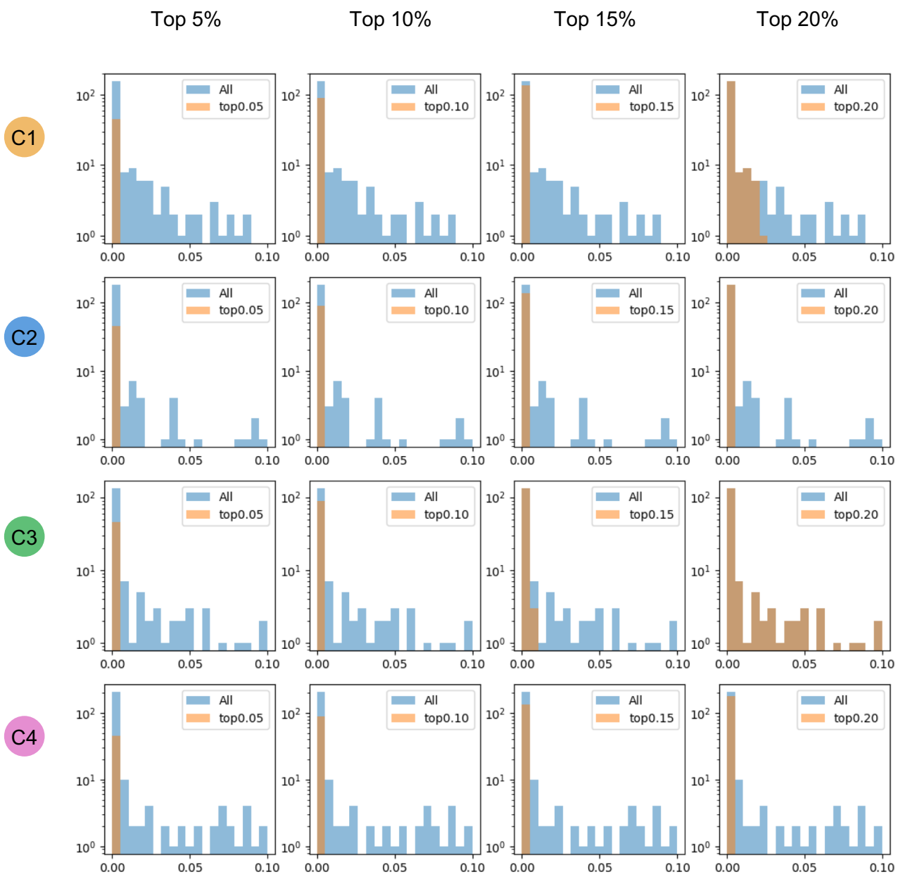
S5 Fig. Variable network PCC cutoff selection. 5%, 10%, 15%, and 20% were used to test the K% connections with the highest PCC for the construction of the network
