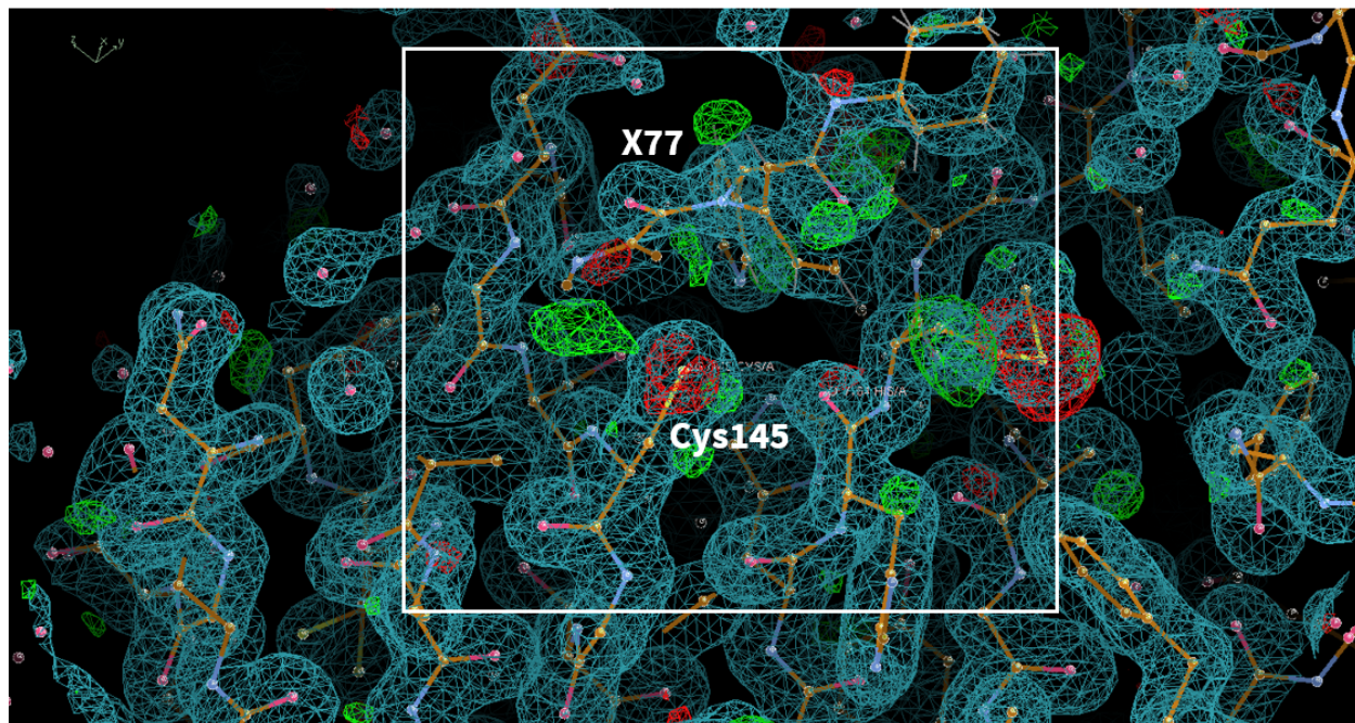
Figure S5 Representation of the 2Fo-Fc electron density map of SARS-CoV main protease (PDB ID: 6W79). Related to Figure 5.
