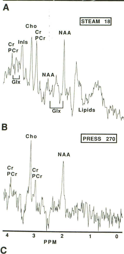
Fig. 7. Image-guided single-voxel proton MRS using a 3.4-cc voxel ( square ) of interest chosen from axial brain MR images of a 12-month-old boy with an unknown metabolic disease affecting cerebral white matter.
