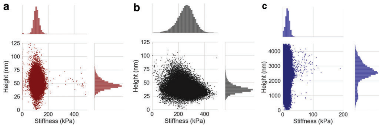
SUPPLEMENTARY FIG. S3. Analysis of fibronectin and matrigel substrates and height versus stiffness scatterplots. (a–c) Representative height versus stiffness scatterplots for complete coating of (a) matrigel, (b) fibronectin, and (c) cluster of cell bodies of cell monolayer.
