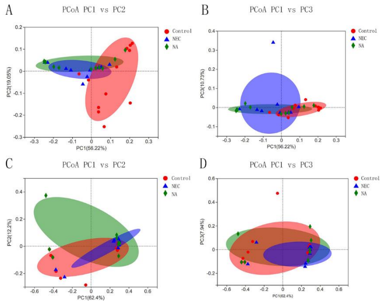
Supplementary Figure 3. PCoA based on weighted and unweighted UniFrac distances. (A and B) PCoA results based on the weighted UniFrac distance. (C and D) PCoA results based on the unweighted UniFrac distance. PC- percent variance explained.
