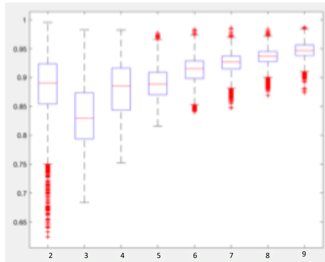
Concordance Index
