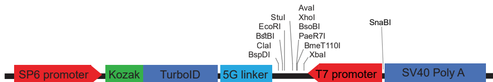
pCS2+ TurboID
