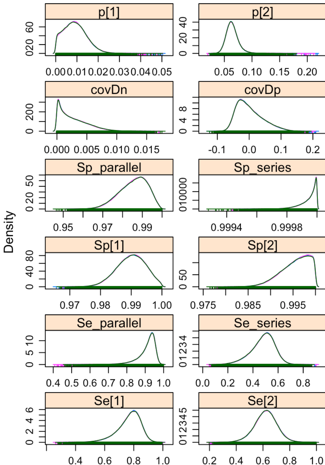
S4 Fig. Density plots of cattle model parameters. Cattle data are from the combined BacZoo study conducted 2013 to 2015 in Arusha and Kilimanjaro Regions, and the SEEDZ study conducted in 2016 in Arusha and Manyara Regions of Tanzania. p[1] denotes seroprevalence in the non-pastoralist subpopulation. p[2] denotes seroprevalence in the pastoralist subpopulation. Se is sensitivity. Sp is specificity. [1] denotes the Rose Bengal plate test. [2] denotes the Animal and Plant Health Agency, UK, competitive enzyme-linked immunosorbent assay. series is a series diagnostic testing approach. parallel is a parallel diagnostic testing approach. covDn is covariance when animal is disease negative. covDp is covariance when animal is disease positive.
