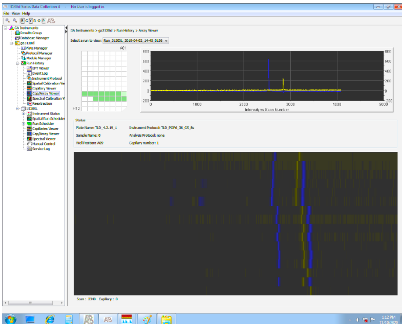
Figure S1: Variability between retention times of products in different capillaries. A screenshot from the 3130XL Data Collection software in the capillary array viewer is shown. FAM peaks are shown in blue and Cy3 internal standard peaks are shown in yellow. The experiment shown has two peaks, however the retention time varies between capillaries.
