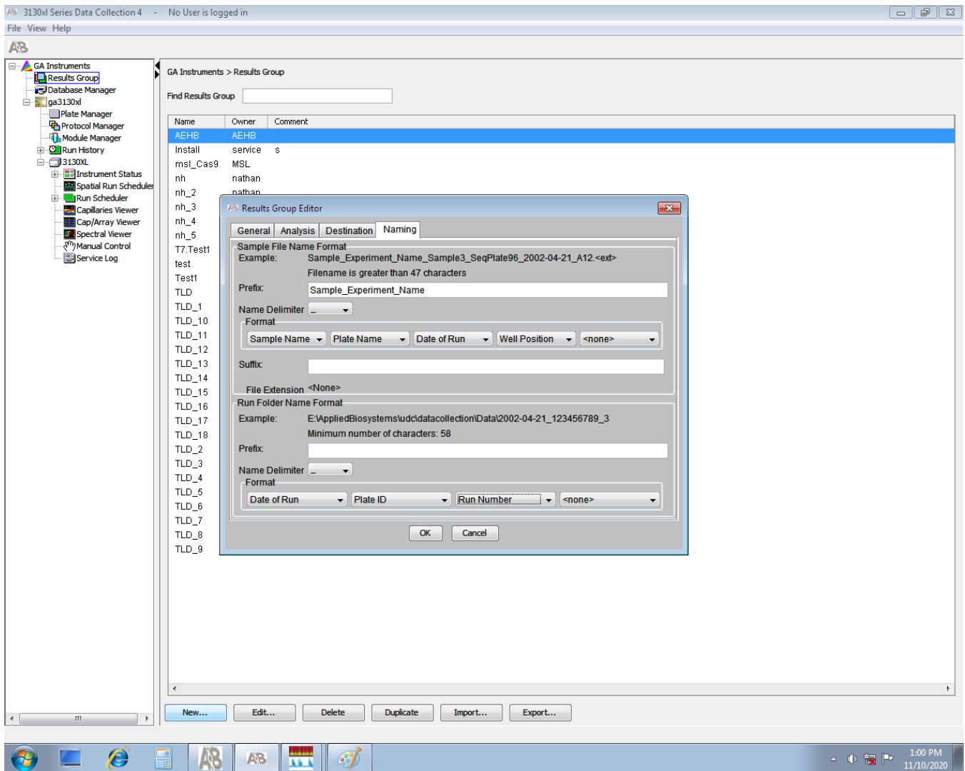
Figure S2: Results Group Editor Settings: Suggested settings for the results group are shown in the results group editor for the 3130XL Data Collection software. Any values can be input in the general, analysis, and destination tabs. In the naming tab, it is important the Name delimiter be set to _ and that the sample name appears in the format for the sample file name. This is needed for subsequent analysis using our software.
