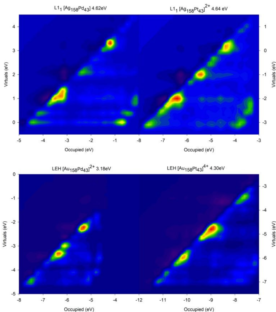
Figure S6. Second set of ICM-OS plots of the closed-shell \text{Ag}_{158}\text{Pd}_{43} , [\text{Ag}_{158}\text{Pt}_{43}]^{2+} , [\text{Au}_{158}\text{Pd}_{43}]^{2+} and [\text{Au}_{158}\text{Pt}_{43}]^{4+} NPs, corresponding to the peak position indicated by the central arrow for each color in Figure 6. The excitonic energy of the analyzed peak is given above each plot.
