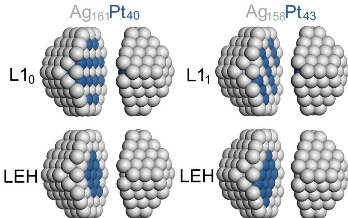
Figure S1. Sketches of 201-atomic AgPt NPs with different atomic orderings. The structures are calculated in J. Phys. Chem. C 2019 , 123 , 25482; doi: 10.1021/acs.jpcc.9b07382. The images are split to show inner parts of the NPs. Ag atoms – grey; Pt atoms – dark blue.
