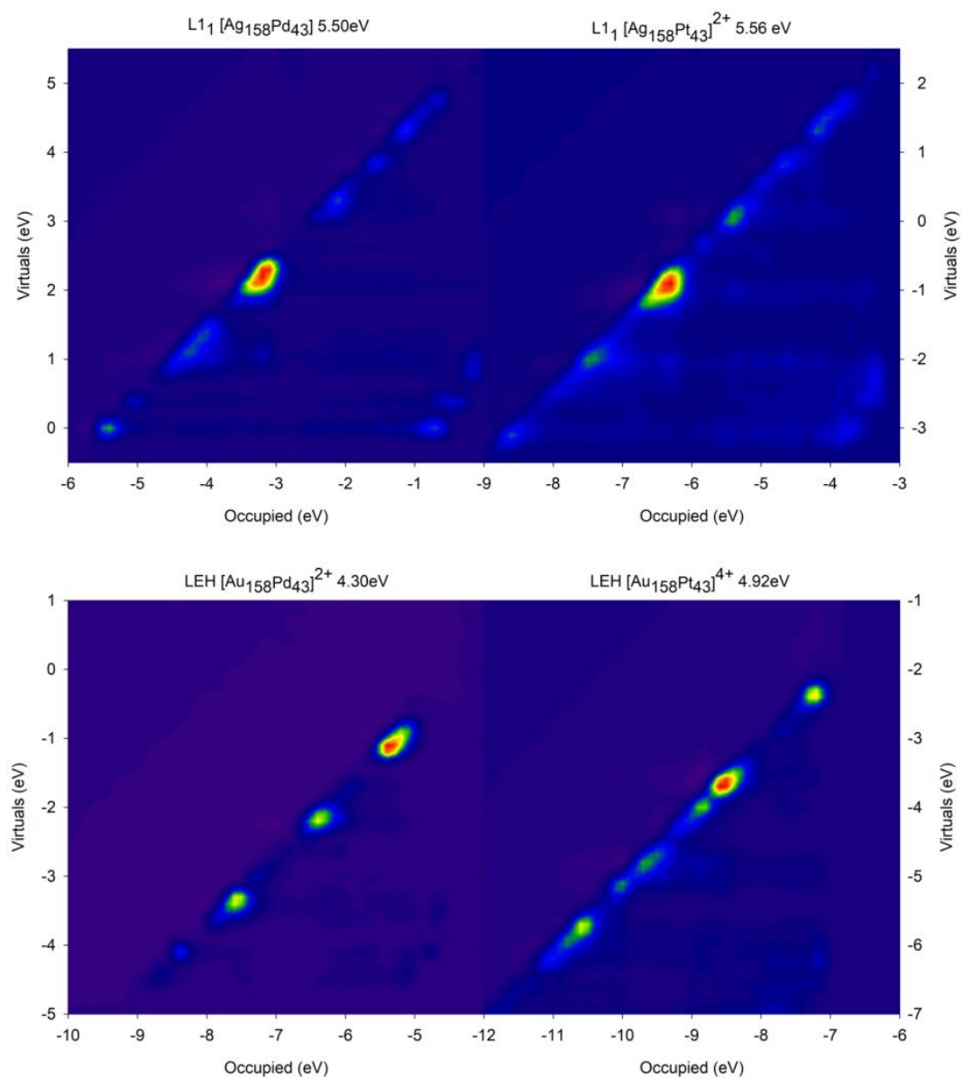
Figure S7. Third set of ICM-OS plots of the closed-shell \text{Ag}_{158}\text{Pd}_{43} , \text{Ag}_{158}\text{Pt}_{43} , \text{Au}_{158}\text{Pd}_{43} and \text{Au}_{158}\text{Pt}_{43} NPs, corresponding to the peak position indicated by the right-most arrow for each color in Figure 6. The excitonic energy of the analyzed peak is given above each plot.
