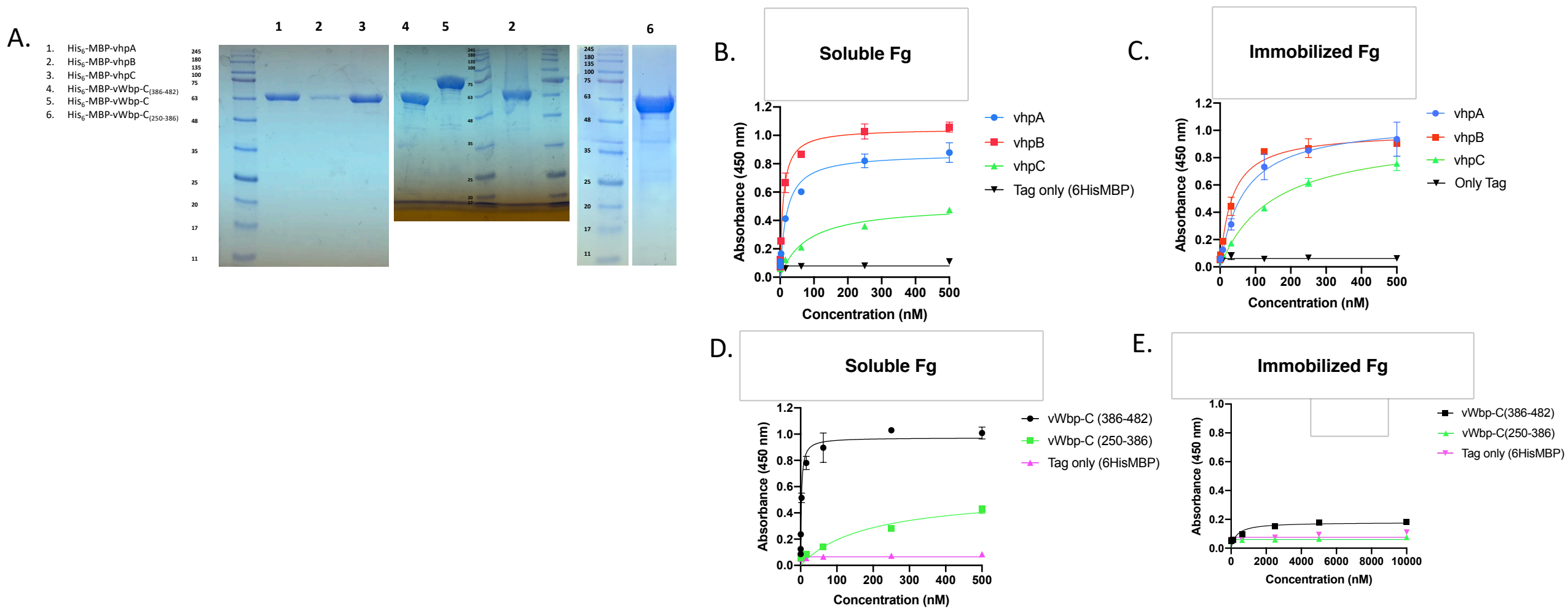
Fig S2. Both vWbp-C (386-482) and vhp bind Fg. (A) SDS-PAGE gel of vhp isoforms and vWbp-C constructs. (B) ELISA binding of soluble Fg to immobilized vhp isoforms (0.5 \mu\text{g}/\text{well} ). (C) ELISA binding of vhp isoforms to immobilized Fg (0.5 \mu\text{g}/\text{well} ). (D) ELISA binding of soluble Fg to immobilized vWbp-C constructs (0.5 \mu\text{g}/\text{well} ). (E) ELISA binding of vWbp-C constructs binding to immobilized Fg (0.5 \mu\text{g}/\text{well} ). Error bars, standard error of the mean (SEM). The graphs are representative of three independent experiments.
