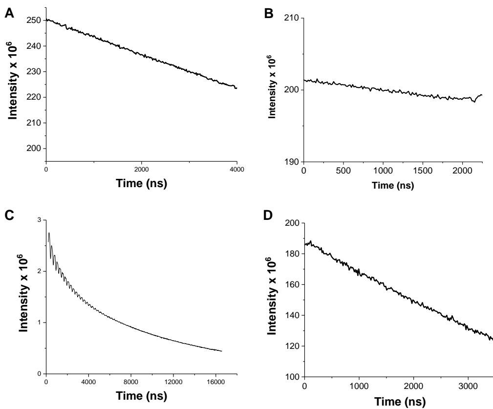
Supplementary Fig. S5. DEER and spin echo signals. (A) DEER signal for UL31 (C1-50) in membranes. (B) DEER signal for UL34 (174-194) in membranes (C) Spin echo signal for UL31 (C1-50) in membranes. (D) DEER signal for UL31 (C1-50) /UL34 (174-194) in solution.
