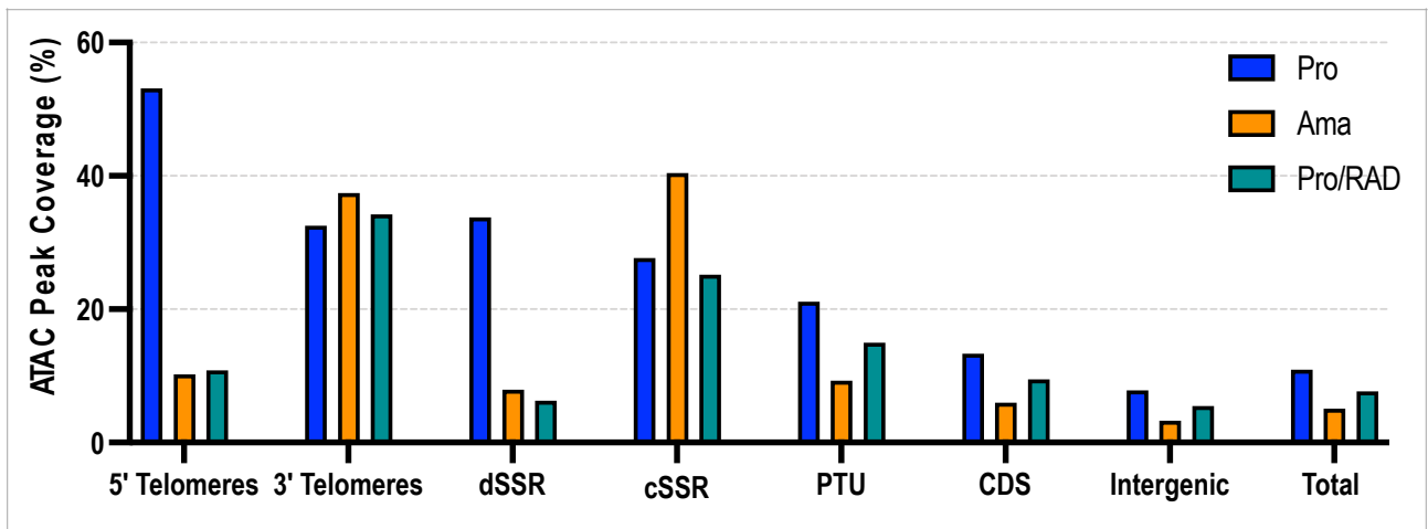
Figure S2. Distribution of open chromatin across the L. donovani genome. Coverage of ATAC peaks is indicated for promastigotes (Pro, blue), axenic amastigotes (Ama, orange) and RAD-treated promastigotes (Pro/RAD, green) at 5'- and 3'-telomeres, divergent (dSSRs) or convergent strand switch regions (cSSRs), polycistronic transcription units (PTUs), coding sequences (CDSs), intergenic regions within PTUs and total chromosomes. Data were pooled from 2 biological samples.
