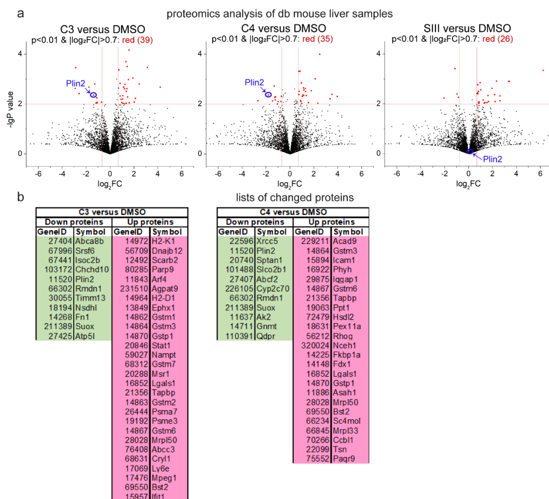
Fig. S8 Proteomic analyses of compound injected liver samples. a Volcano plots of the proteomic analyses of liver samples from mice injected with C3, C4 or SIII versus the DMSO control for 14 days (4 mice per group). Only the proteins detected in at least one sample in each group of the comparison were plotted to avoid error in calculating the \log_2 fold changes ( \log_2FC ) and or the -\log_{10}P values ( -\lgP values). The LD marker protein Plin2 was indicated by the blue circle and arrow in each plot. The statistical analysis was performed for two-tailed unpaired t test. b The tables and Venn diagram illustrating significantly changed proteins for each comparison ( |\log_2FC| > 0.8 and p < 0.01 ). See Data S2 for detailed data used for the analysis and plots.
