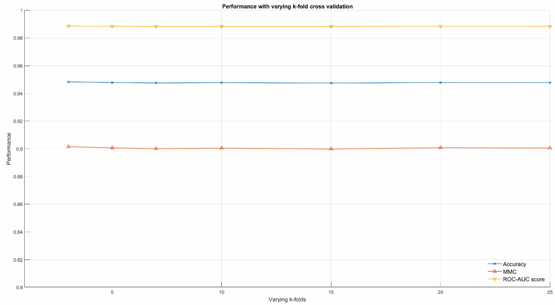
Figure S1 Performance with varying k -fold cross validation ( k=3, 5, 7, 10, 15, 20, 25 ) in terms of Accuracy, MCC and ROC-AUC score.
