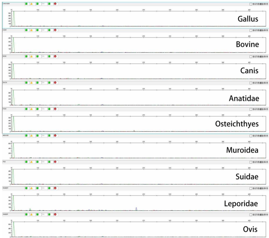
Figure S1. Electropherograms from species specificity studies of the AGCU X-InDel 38 kit.
