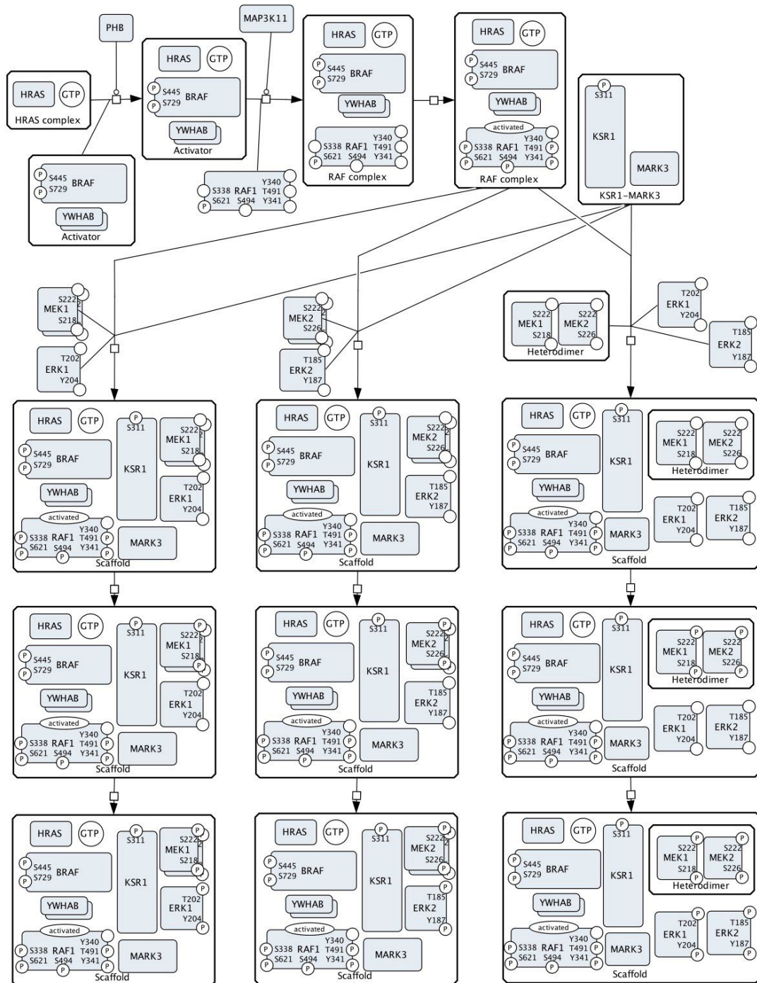
Supplementary Figure S2. An inferred CellDesigner's view alternative to Figure 3a - the RAF/MAP Kinase Cascade map (Pathway:R-HSA-5673001) from the Reactome pathway database ( https://reactome.org ) [Jassal 2020 PMID:31691815; Fabregat 2018 PMID:29377902].
