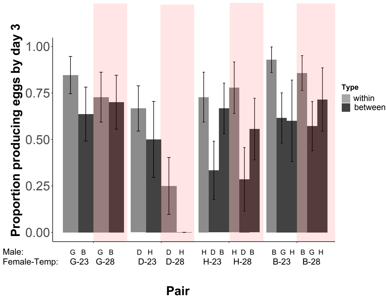
Appendix Figure 1. Proportion of pairs producing eggs by male line, female line, and temperature. Male line listed above, female line and temperature listed below. DV females were less likely to produce eggs than BV females at high temperature. Bars represent standard error of the proportion. Light gray = within-line pairs, dark gray between lines = between-line pairs, 28°C pairs shaded in red. No interactions between female line and temperature were significant. G = GE/Geneva D = DV/Dover; H = HR/Hurley, B = BV/Bouckville.
