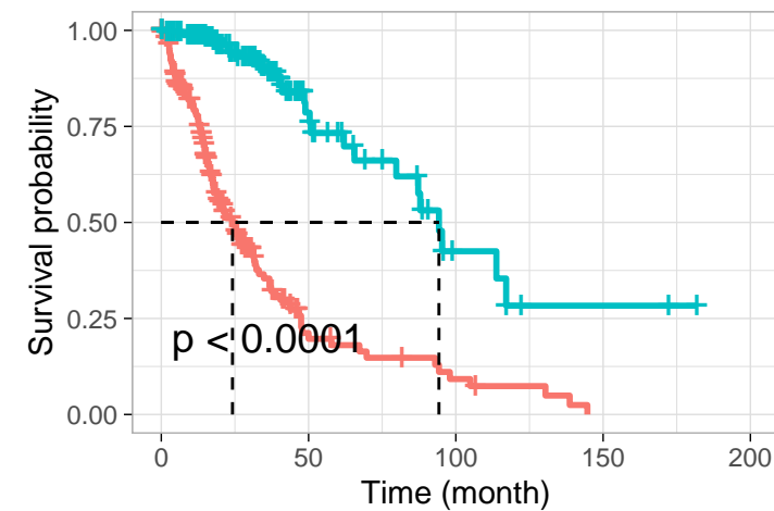
PYGL OS in TCGA (IS3)
