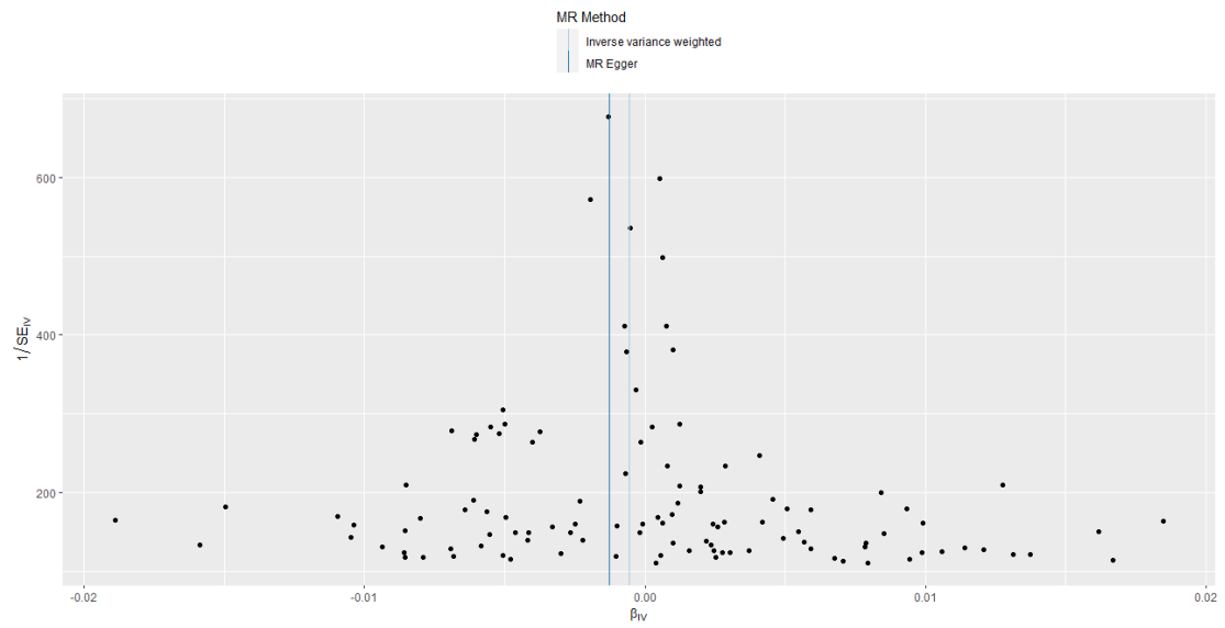
Funnel plot for total cholesterol
