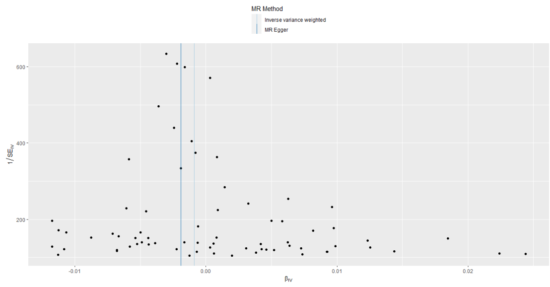
Funnel plot for triglycerides
