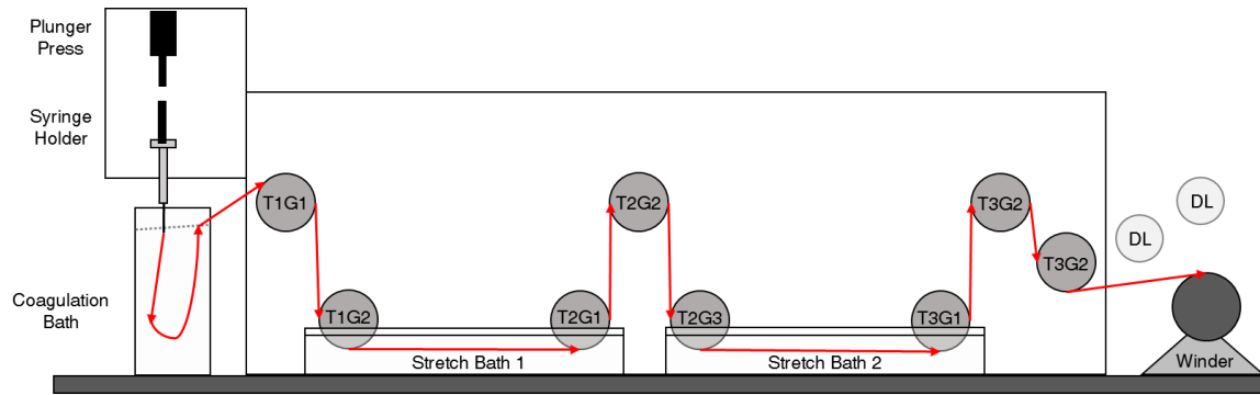
Fig. S4. Diagram of customized extrusion method and spinning instrument.
