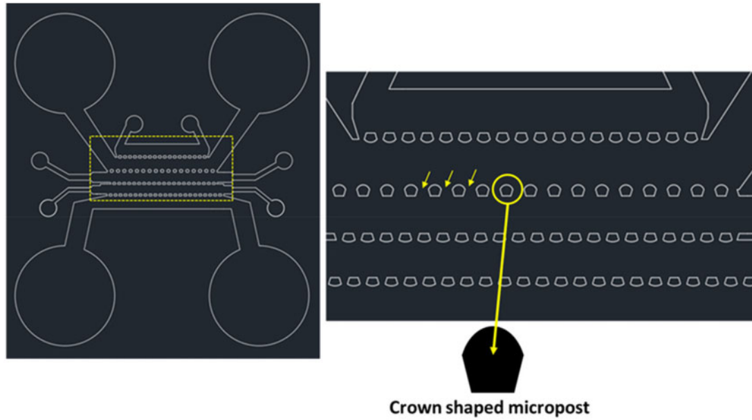
Supplementary Figure S1. Computer-aided design (CAD) of microengineered vascularised endometrium-on-a-chip. The microfluidic platform consists of five parallel channels.
