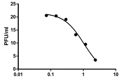
\delta B.1.617.27/S:478K
