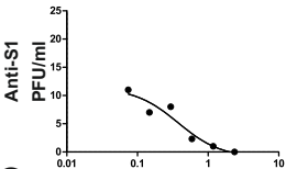
Ger-EPI-ISL-406862
