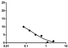
\beta B.1.351/501Y.V2
