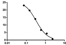
\epsilon B.1.427/B.1.429
