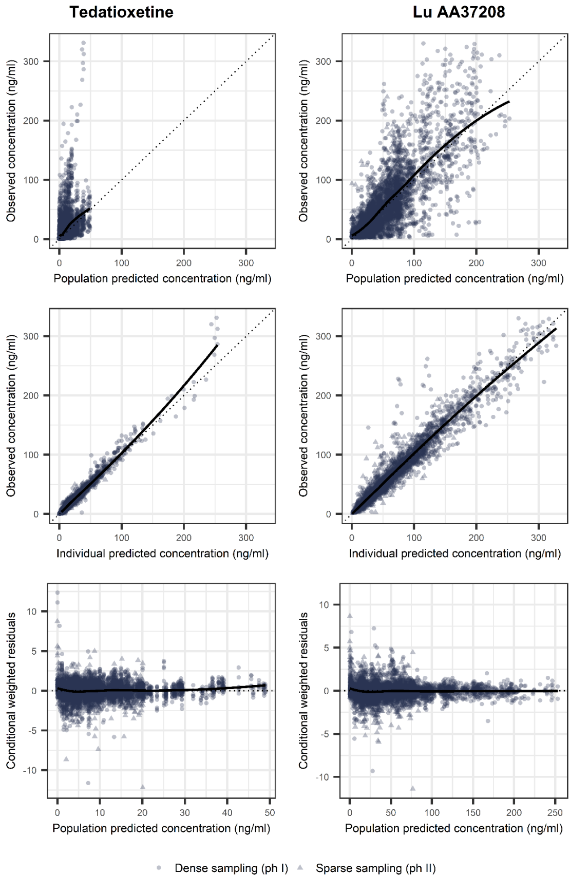
Figure S1 Goodness-of-fit plots for the final population pharmacokinetic model for tedatioxetine and Lu AA37208. Shapes indicate whether the data is based on dense (circles) or sparse (triangles) pharmacokinetic sampling
