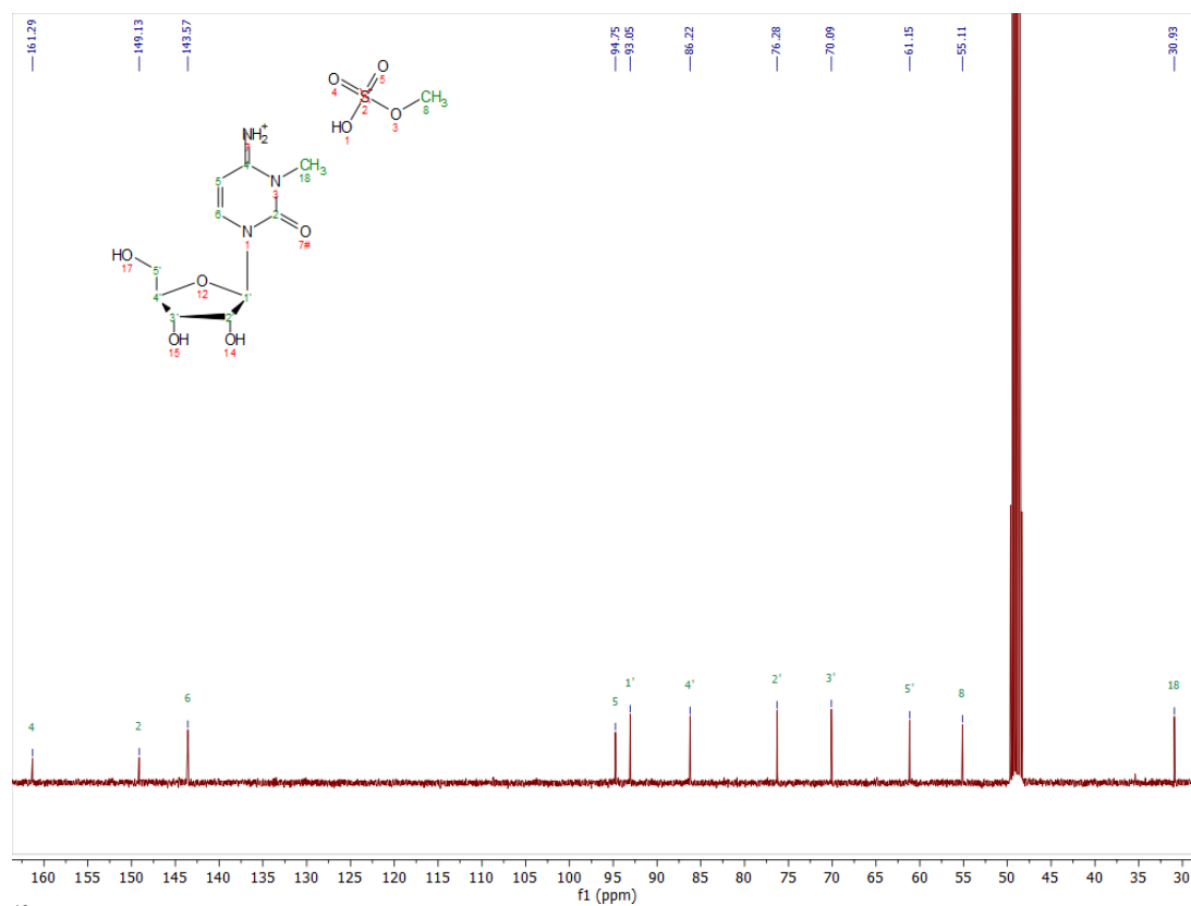
13 C-NMR (100 MHz, MeOD) of compound 1.
