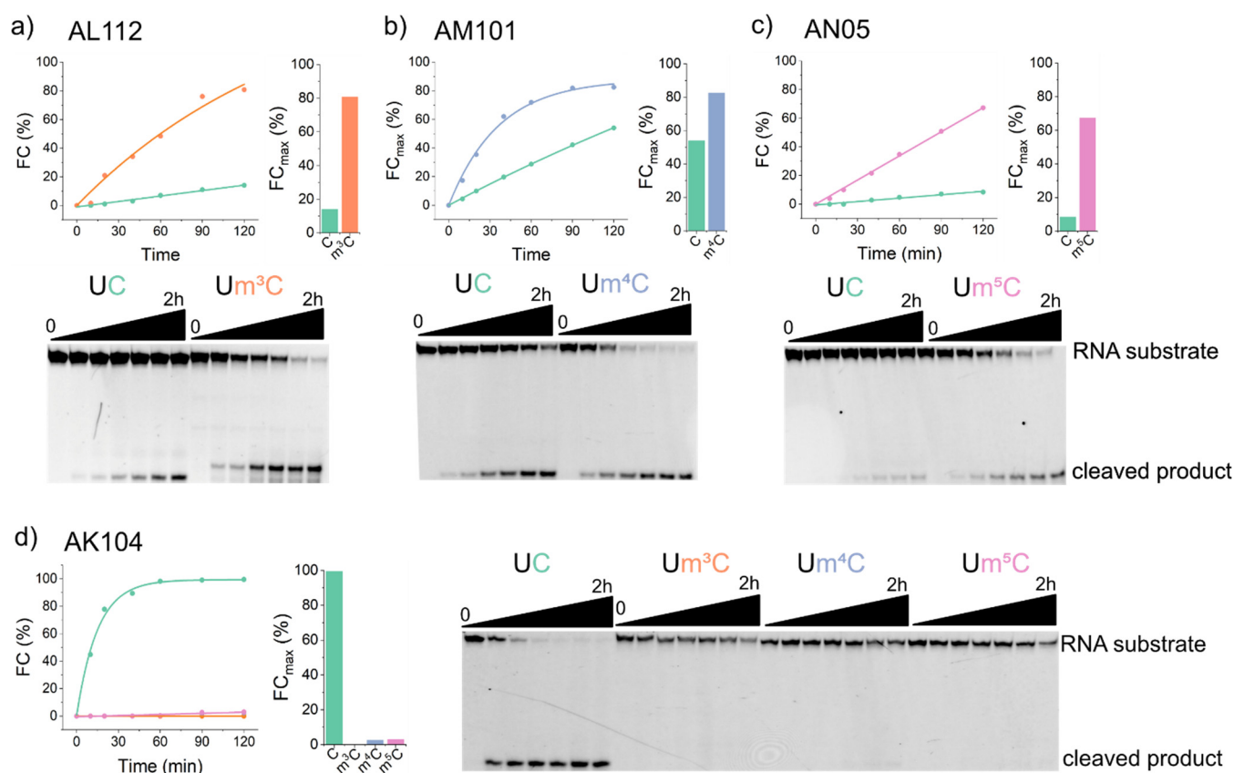
Figure S13. Cleavage activity of deoxyribozymes AL112, AM101, AN05 and AK104 in the presence of Mn 2+ . a)–c) Top panel: kinetic plots and comparison of FC values obtained after 2 h cleavage for deoxyribozymes AL112, AM101 and AN05, respectively. Bottom panel: gel images for cleavage of R8 and R12 with AL112 (a), R8 and R16 with AM101 (b), R8 and R20 with AN05 (c). d) kinetic plots and comparison of FC values obtained after 2 h cleavage for deoxyribozyme AK104 (left). Gel image for cleavage of R8, R12, R16 and R20 with AK104 (right). Conditions: 100 pmol deoxyribozyme, 10 pmol RNA substrate, 20 mM MnCl 2 , 50 mM Tris-HCl, 150 mM NaCl, pH 7.5, 37 °C, 2 h.
