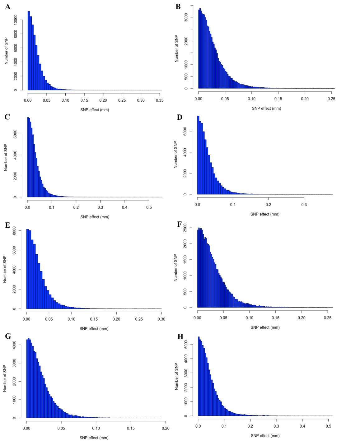
Figure S1. Distribution of the SNP effects on backfat thickness (mm) in the eight pig lines.
