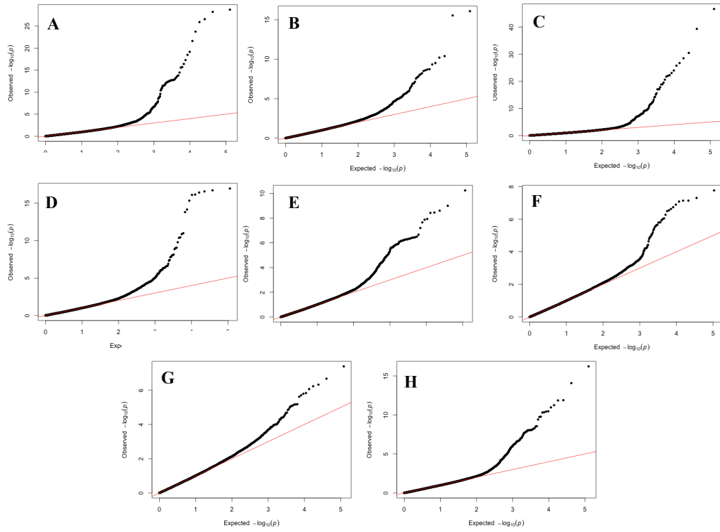
Figure S2. Q-Q plots for the genome-wide association study of backfat thickness for the eight pig lines.
