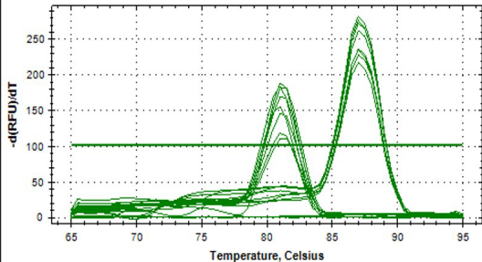
Melt Peak
