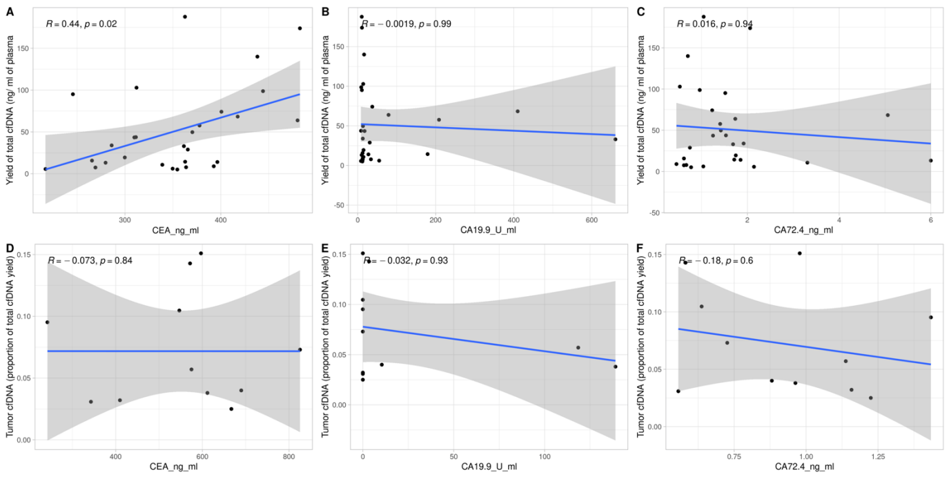
Supplementary Figure 1. Spearman's correlation analysis between level of oncoproteins CEA, CA 19-9, CA 72-4 (x-axis), and total circulating cfDNA (a-c) and tumor derived cfDNA yield (d-f). Moderate positive correlation was determined between levels of CEA (ng/ml) and total cfDNA yield ( R = 0.44, p = 0.02 )
